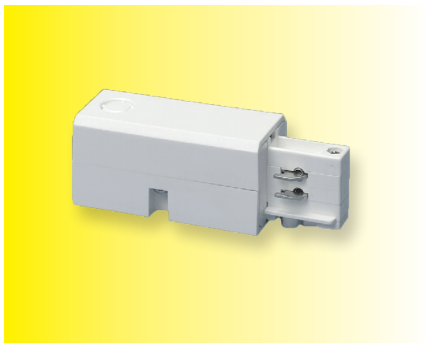
EURO-TRACK Einspeisung (L) EURO-TRACK Alimentation (G)
